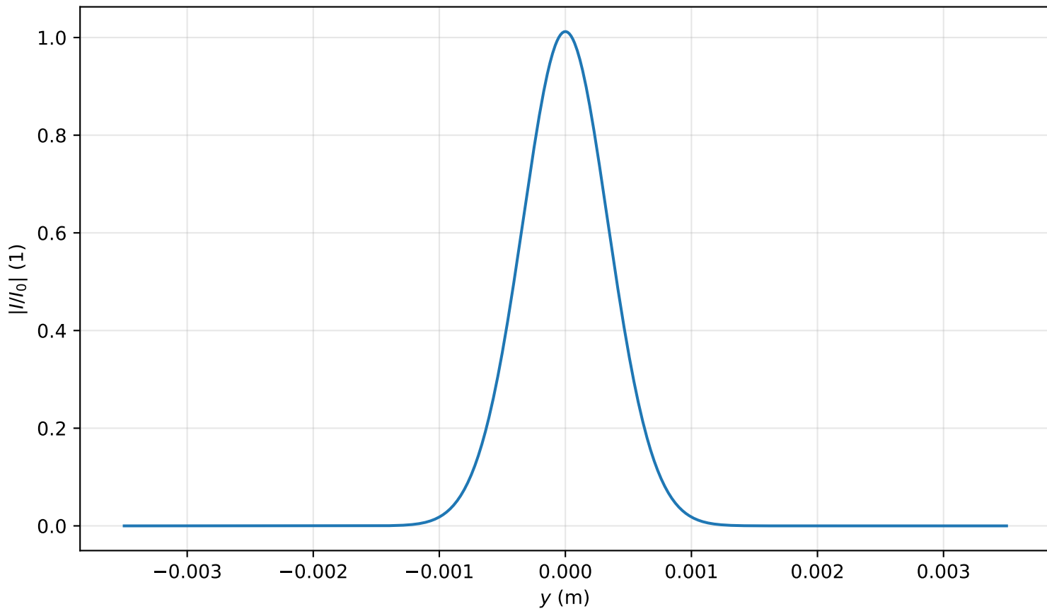
Intensity profile I(x=0, y, z=0.318)/I_0 , P_{in}=0.4P_{cr} , artificial time
